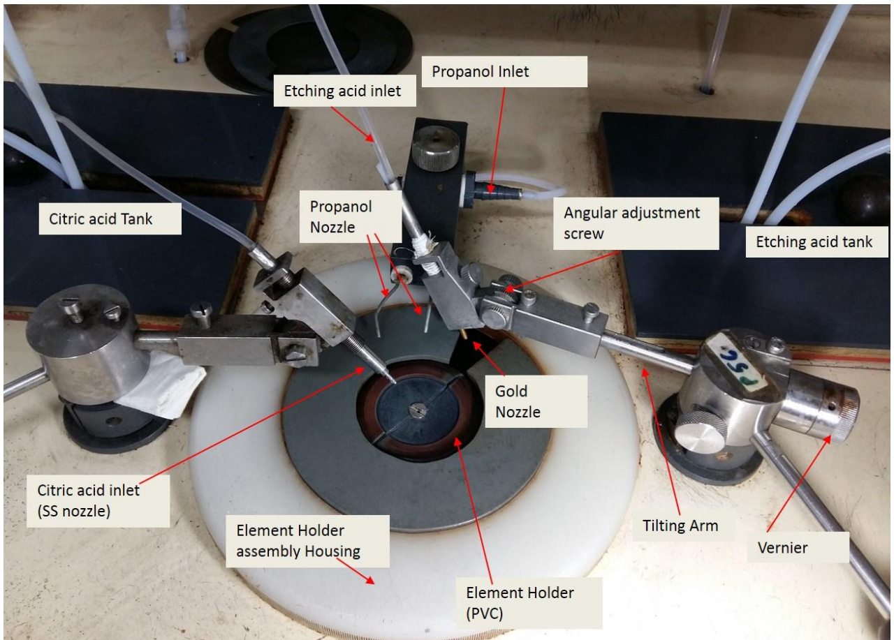
PICTURE-2: ELEMENT HOLDER AND JIG ASSEMBLY
